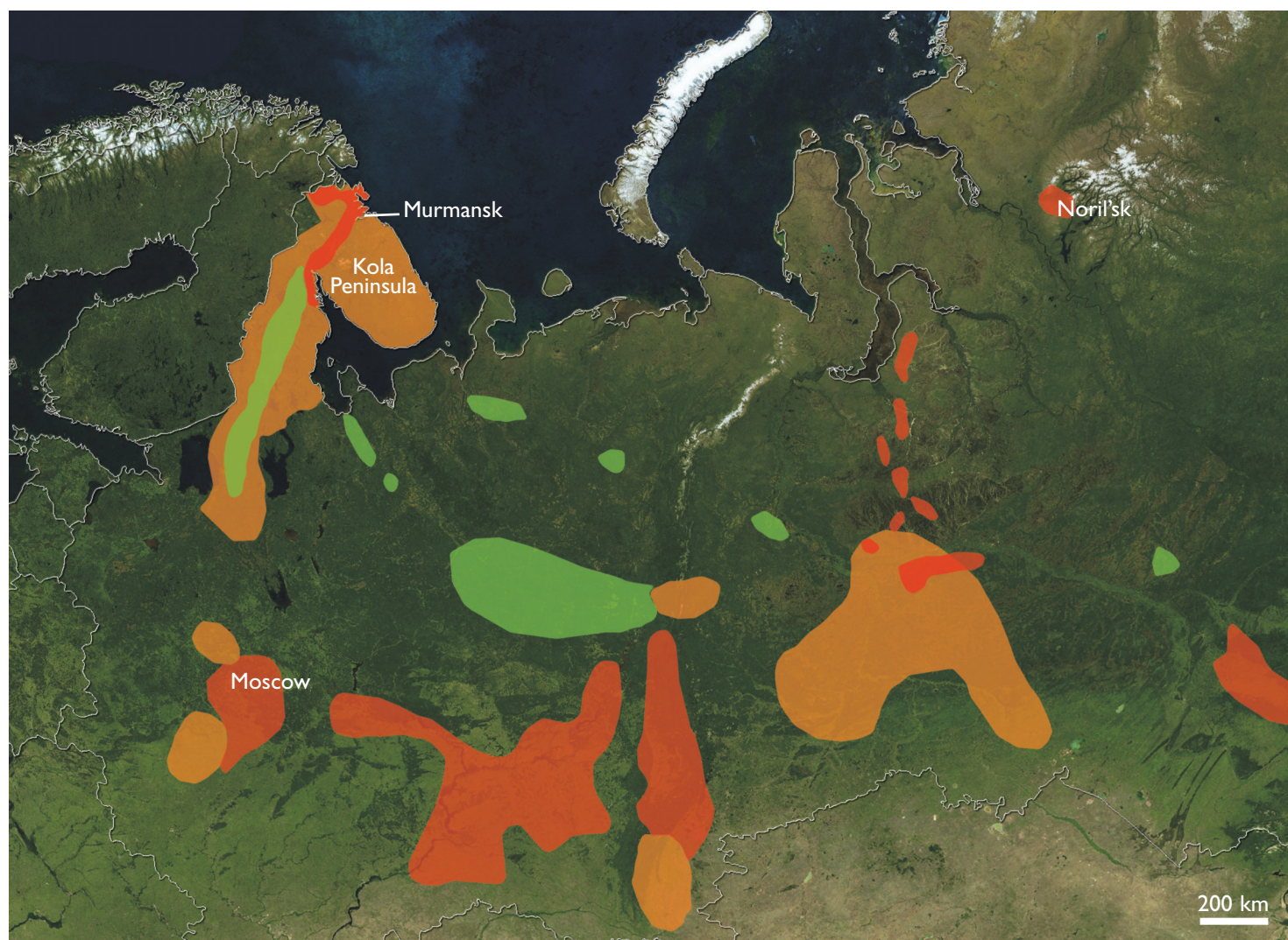
Environmental landscape impacts in the Russian North. Red: critically degraded areas; orange: areas affected by acid rain; bright green: areas of forest damage. (Based on data from the Handbook of International Economic Statistics , 1998.)
