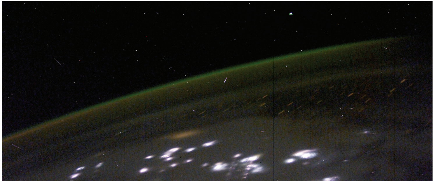
Lightning from a storm system extending from Argentina to southern Brazil on the evening of April 23, 2003. (Photograph from the International Space Station, NASA Image Exchange, image number ISS006-E-48196.)
