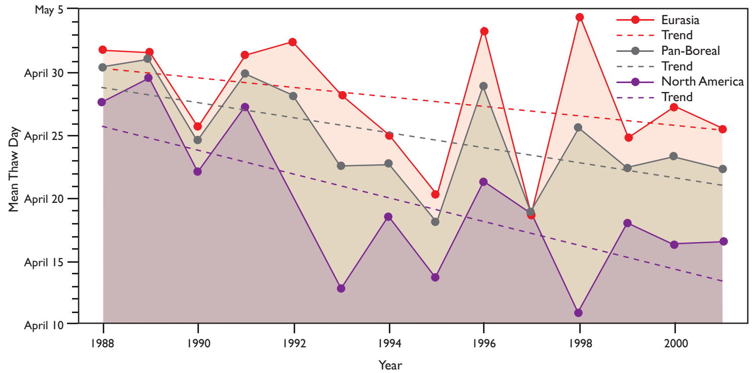
Trend in mean thaw day for the entire pan-boreal region and for North America and Eurasia. North America is experiencing a more pronounced advance in thaw day than is Eurasia. (Data from the SSMI instrument on a DMSP satellite.)
