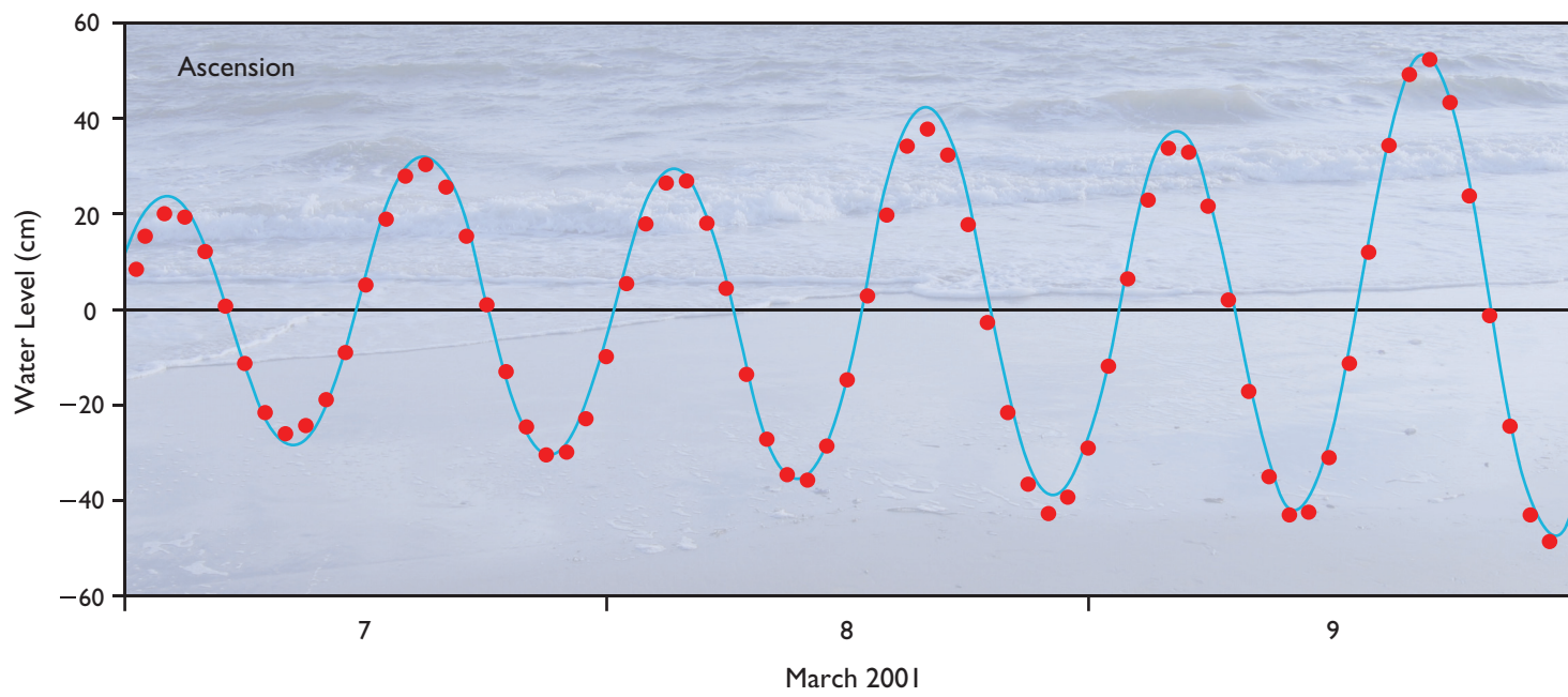
Ground-truth validation of satellite-based tide predictions. A tidal prediction (blue curve), based on analysis of TOPEX/Poseidon satellite altimeter data collected in the vicinity of Ascension Island, in the middle Atlantic Ocean, is found to compare well with actual hourly water level measurements made at the island (red circles.) (Hourly data courtesy Proudman Oceanographic Laboratory, UK.)
