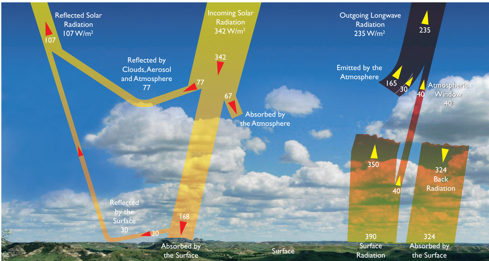
The Earth's annual global mean energy budget at the top-of-atmosphere, surface and within the atmosphere. (Illustration adapted from J. T. Kiehl and K. E. Trenberth, 1997, Bulletin of the American Meteorological Society , vol. 78, pp. 197–208.)
