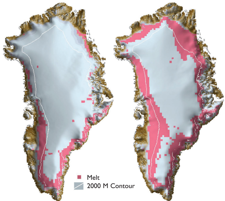
1992 Melt Extent
