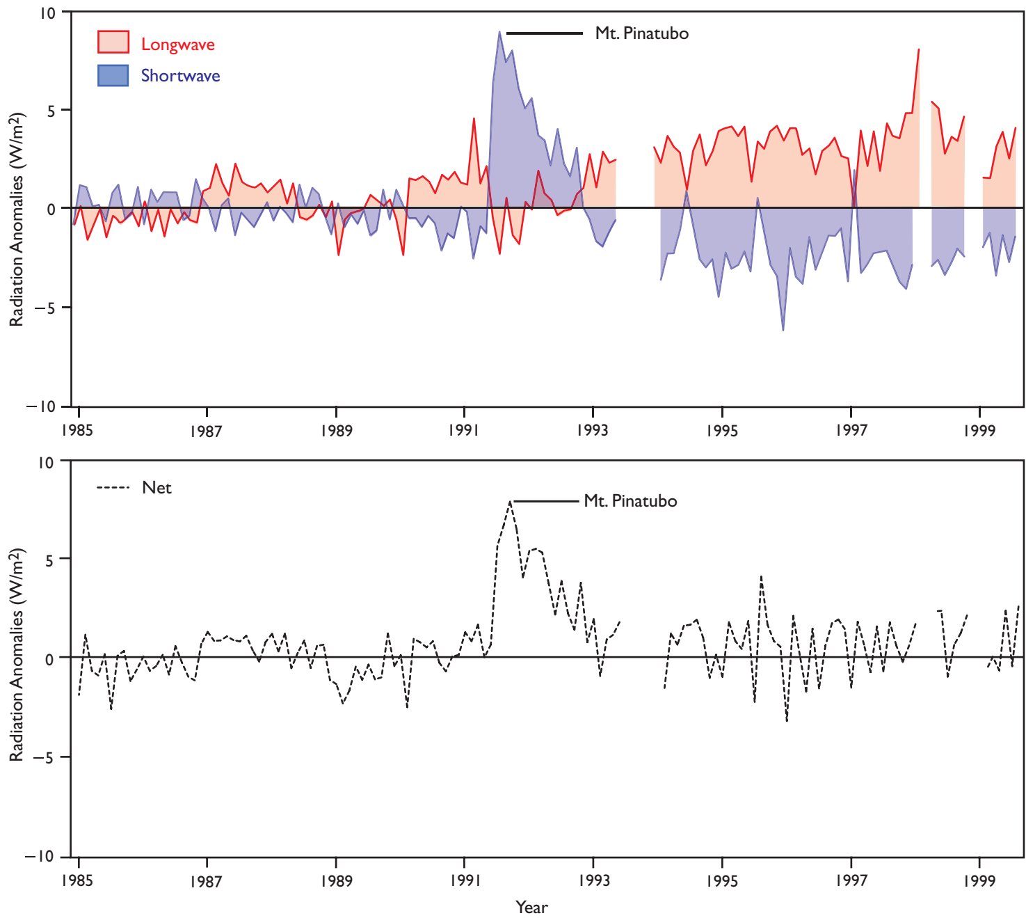
Comparison of the observed longwave (red), shortwave (blue) and net (black) radiation at the top of the atmosphere for the tropics (20°N–20°S) as deviation from the mean for 1985–1990. (Data from the ERBE instruments on the ERBS satellite and the CERES instrument on the TRMM satellite.)
