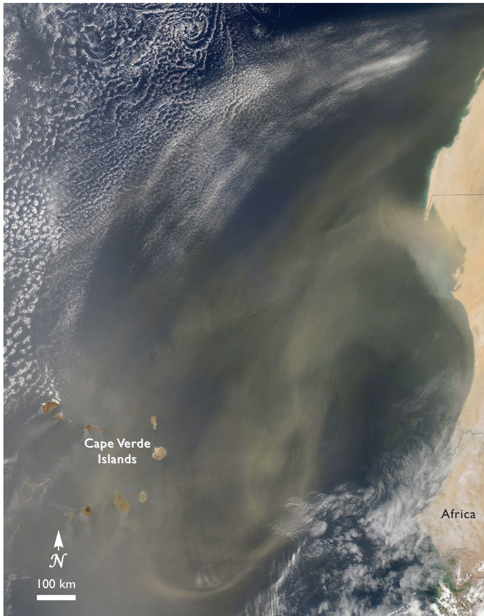
Giant plume of Saharan dust on May 19, 2005, which eventually traveled 1,600 km into the Atlantic Ocean. (Data from the MODIS instrument on the Aqua satellite.)
