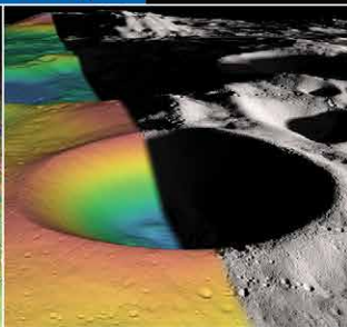
CRATER ON THE MOON
