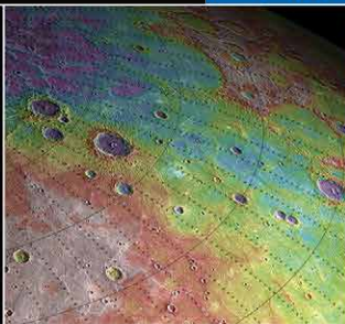
HIGHS AND LOWS ON MERCURY
