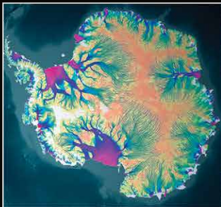
ANTARCTIC ICE FLOW
