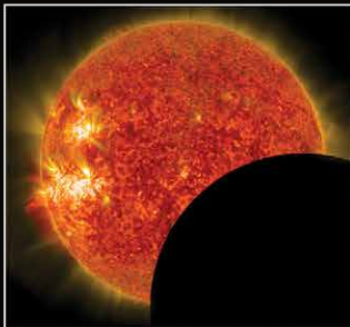
SOLAR ECLIPSE
