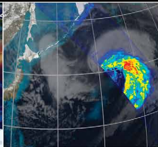
EXTREME WEATHER
