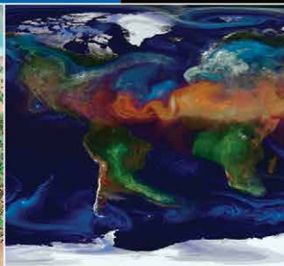
AEROSOLS AROUND THE WORLD
