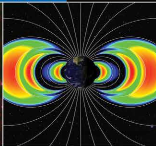
RADIATION BELT AROUND EARTH
