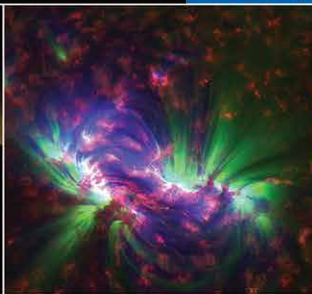
SOLAR WIND
