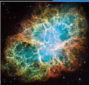
CRAB NEBULA
