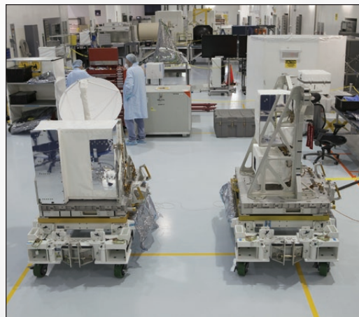
[Above] The components of NASA's ISS-RapidScat payload (i.e., the Instrument and Nadir Adapter) rest side-by-side after removal of their shipping cover inside Kennedy Space Center's Space Station Processing Facility.
