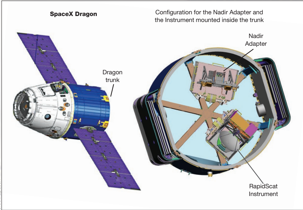
[Above] Prior to launch, the RapidScat Instrument and Nadir Adapter will be strategically mounted inside the Dragon trunk on SpaceX.
